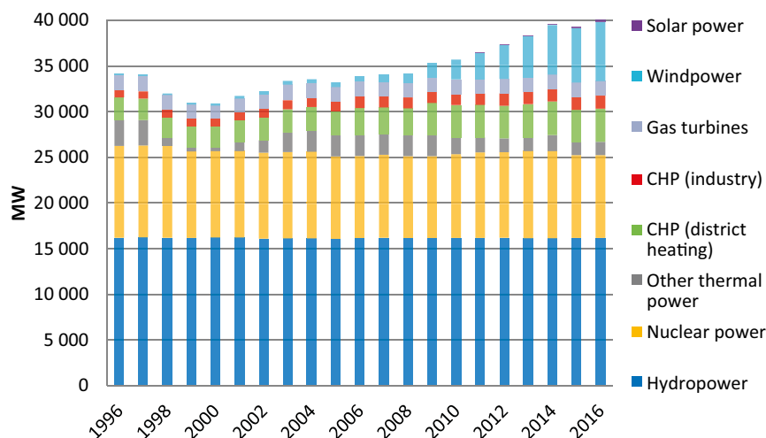
Figure 20 Electricity production capacity, 1996–2016, MW.
